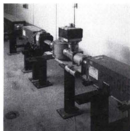
Permanent magnets flank beam monitoring instruments, a vacuum pump and a short "trim" electromagnet for course correction in the 8-GeV Line.
