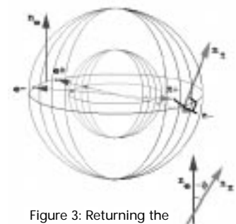
Figure 3: Returning the normal of the e^+e^- plane to its original position.
