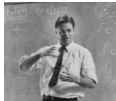
Fermilab Photos
