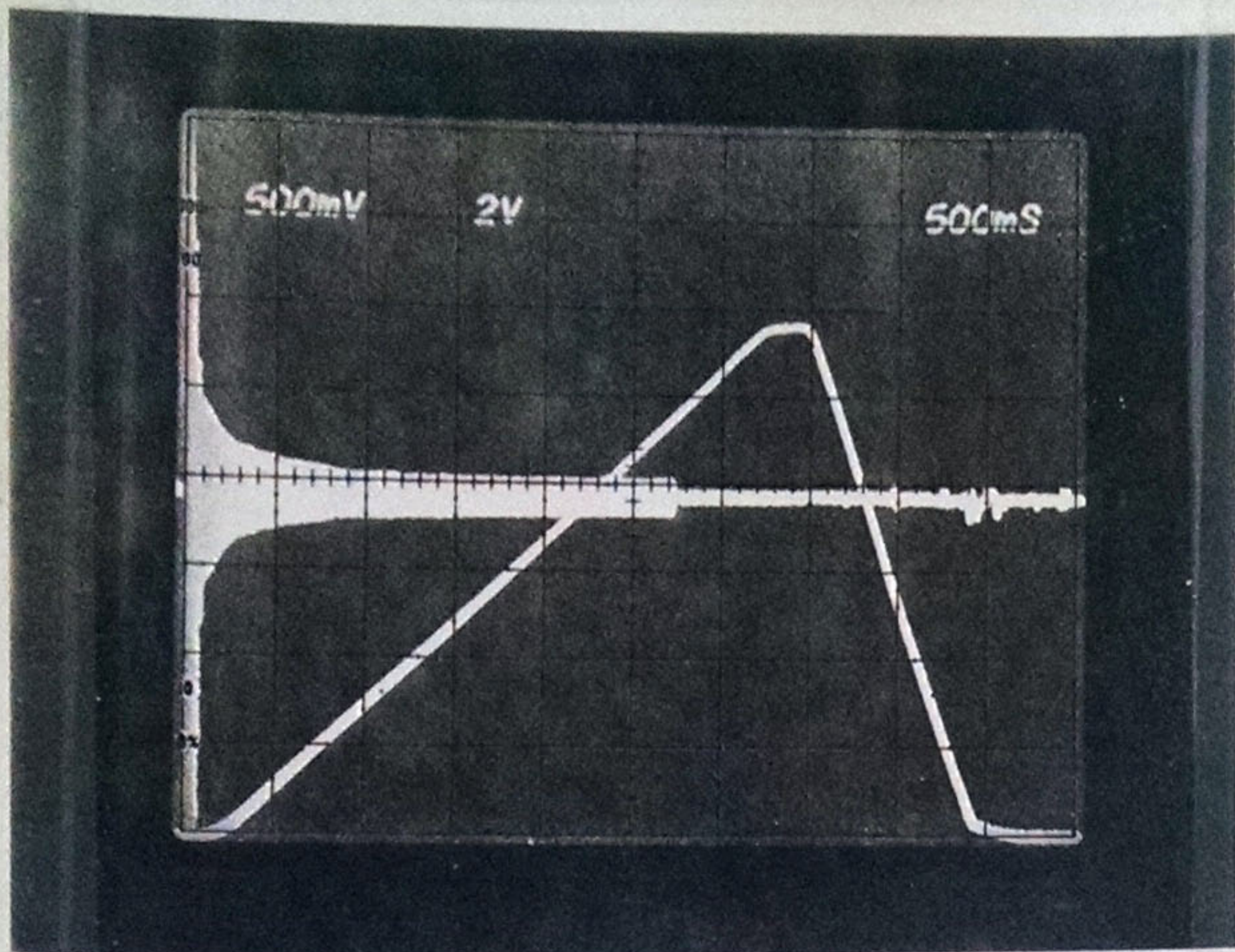
162 BeV 1 March 1972
